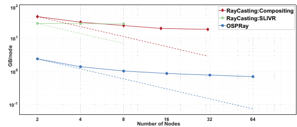
Figure 16: Comparison of the memory footprint when rendering the coal-boiler of VisIt’s RayCasting:Compositing and RayCasting:SLIVR renderers with our OSPray renderer on Stampede2 KNL nodes. We find that moving to the hybrid-parallel model of OSPray comes with a significant reduction in memory use.
