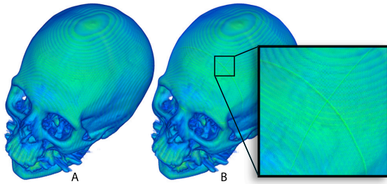
Figure 7: The rendering artifact produced by inconsistent sampling between bricks. A) The CT-head dataset rendered by VisIt-OSPRay using consistent sampling between bricks; B) the same data rendered using OSPRay's built-in volume type, resulting in discontinuities at the brick boundaries.
