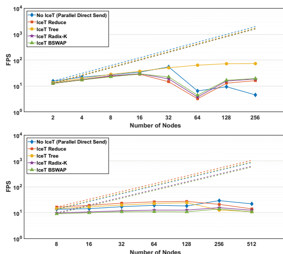
Figure 10: Strong scaling on the coal-boiler dataset using image compositing algorithms available in IceT and VisIt. The benchmarks were run on Stampede2 KNLs (top) and Theta (bottom).
